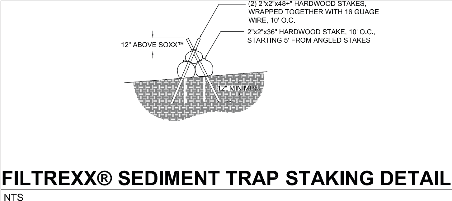
Figure 9.2. Engineer Design Detail for Staking Sediment Traps.
