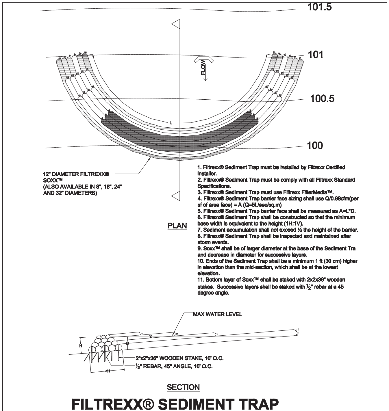
Figure 9.1. Engineer Design Drawing for Sediment Trap.
